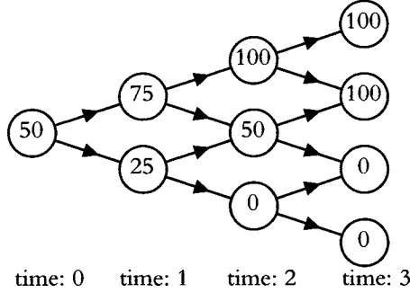
Figure A.1 The option claim tree for a digital payoff
